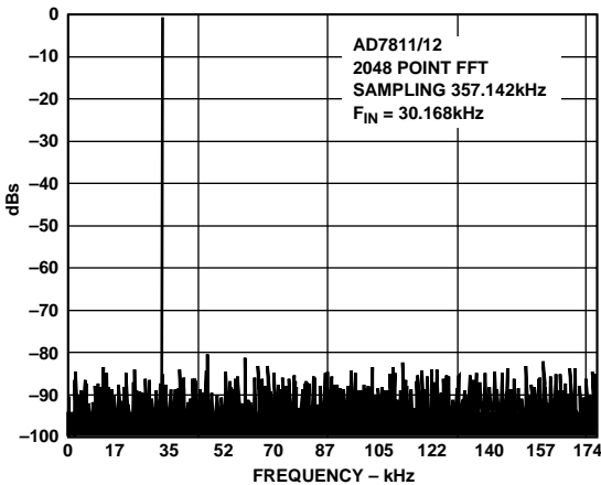
Figure 13. AD7811/AD7812 SNR
