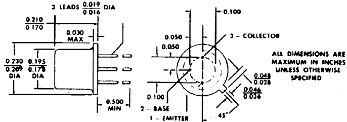
TO-18
