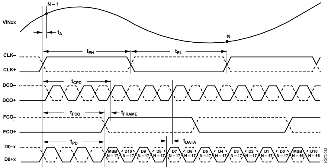
Figure 6. Wordwise DDR, One-Lane, 1x Frame, 12-Bit Output Mode
