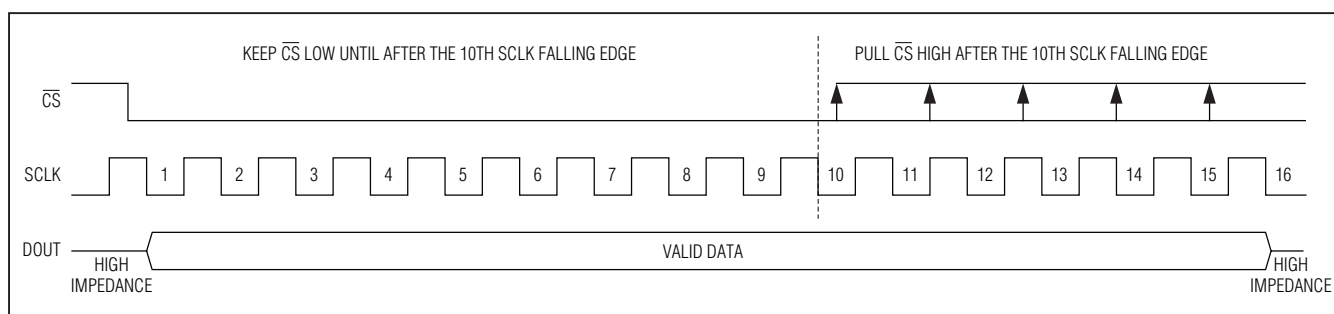
Figure 7. Normal Mode
