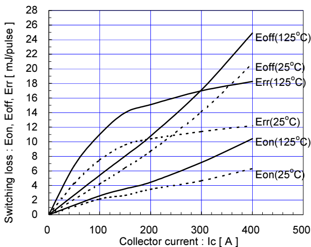
Switching loss vs. Collector current (typ.) V_{cc}=600V, V_{GE}=\pm 15V, R_G=1.6\Omega
