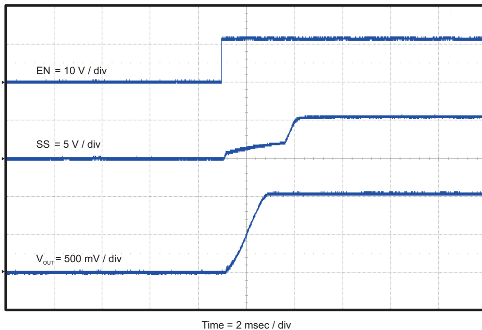
Figure 10. TPS54227EVM-686 Start-Up Relative to EN
