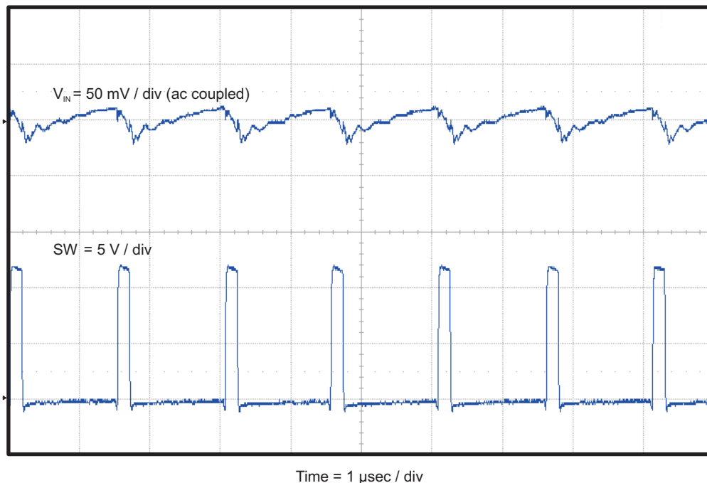
Figure 8. TPS54227EVM-686 Input Voltage Ripple
