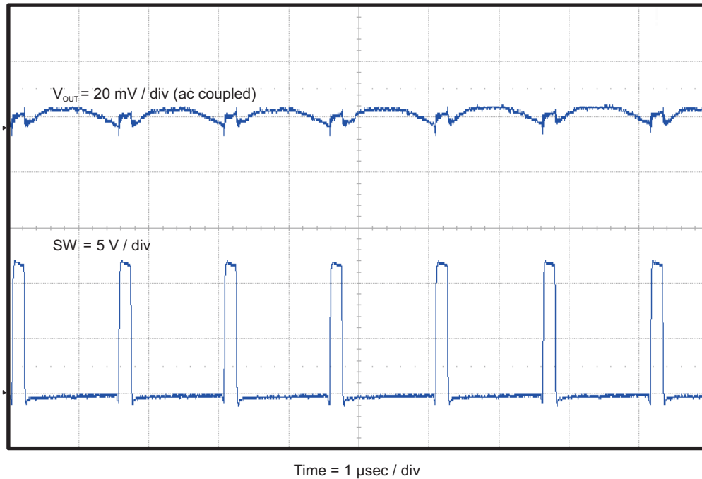
Figure 7. TPS54227EVM-686 Output Voltage Ripple
