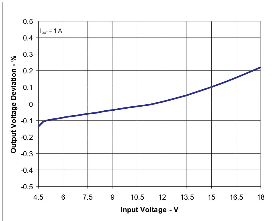
Figure 5. TPS54227EVM-686 Line Regulation
