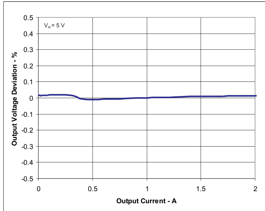
Figure 3. TPS54227EVM-686 Load Regulation, V_{IN} = 5 V.
