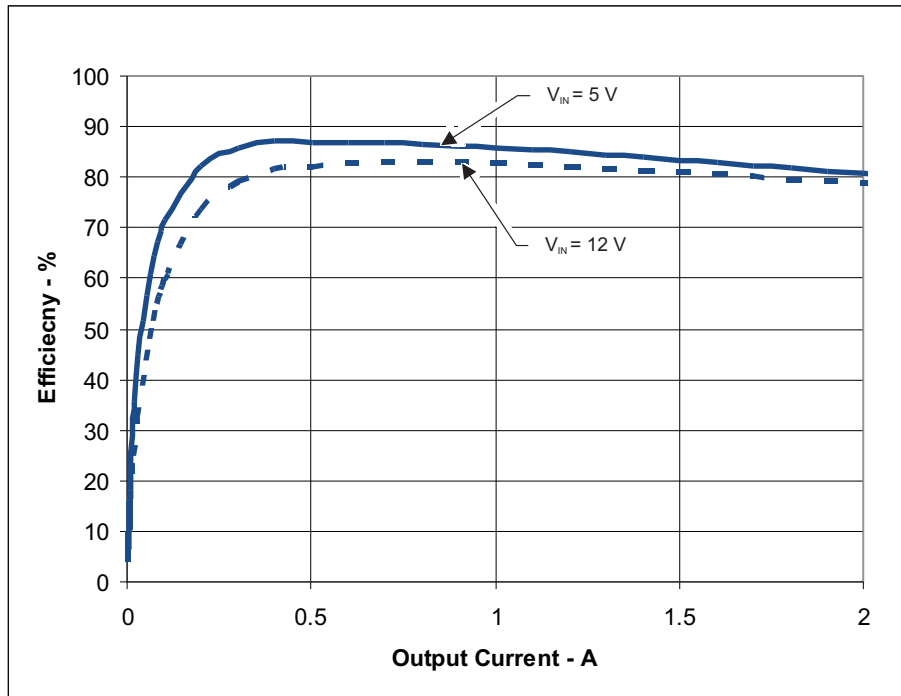
Figure 1. TPS54227EVM-686 Efficiency
