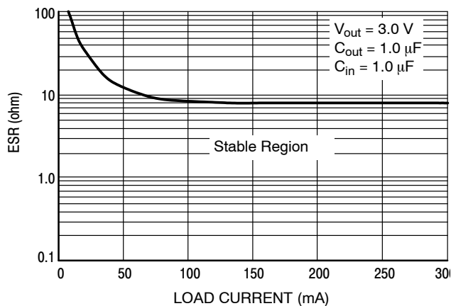
Figure 16. ESR for V_{out} = 3.0\text{V}
