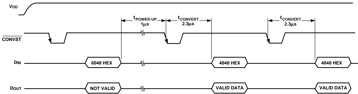
Figure 15. Read/Write Sequence for AD7812
