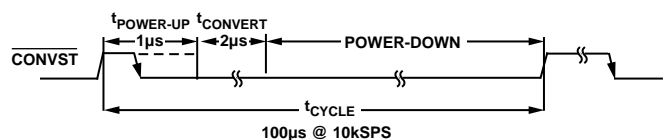
Figure 11. Automatic Power-Down
