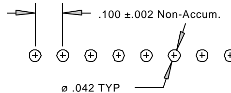
PCB HOLE PATTERN LAYOUT
