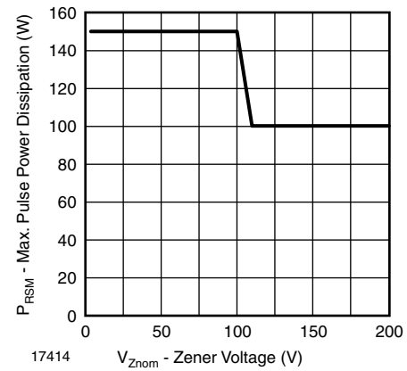
Fig. 4 - Maximum Pulse Power Dissipation vs. Zener Voltage
