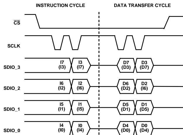
Figure 48. 4-Bit Serial Mode Read Timing—Clock Stall High
