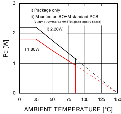
Fig.47 Thermal derating curve (HSOPM28)
