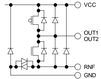
Fig.51 OUT1 / OUT2 (SSOPB24/HSOP25/HSOPM28)
