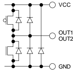
Fig.50 OUT1 / OUT2 (SOP8/HRP7)
