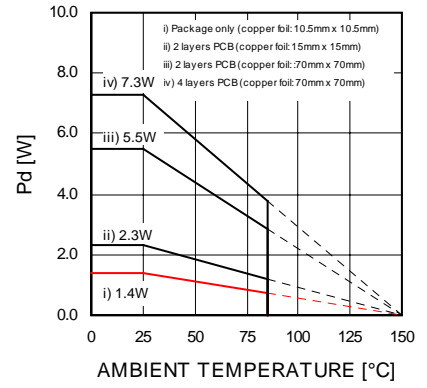
Fig.45 Thermal derating curve (HRP7)
