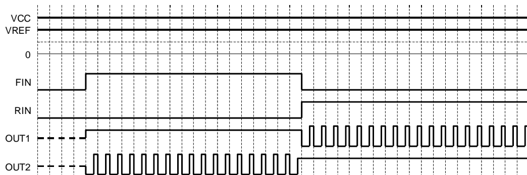
Fig.41 VREF control operation (timing chart)
