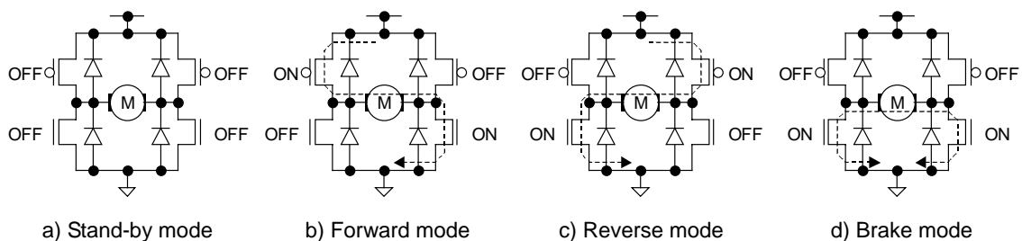
Fig.38 Four basic operations (output stage)
