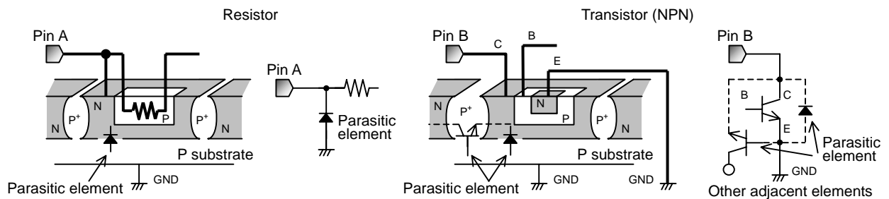
Appendix: Example of monolithic IC structure
