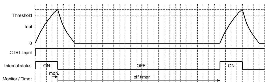
Fig.42 Over current protection (timing chart)
