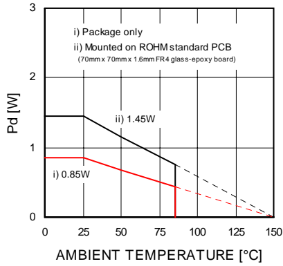
Fig.46 Thermal derating curve (HSOP25)
