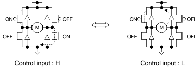
Fig.39 PWM control operation (output stage)
