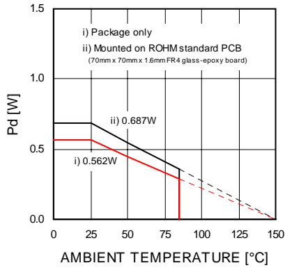
Fig.43 Thermal derating curve (SOP8)
