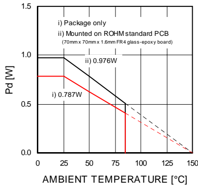
Fig.44 Thermal derating curve (SSOPB24)
