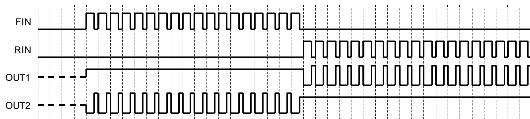
Fig.40 PWM control operation (timing chart)
