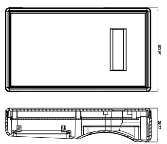
TOP-(MDL-S-16265)
