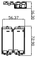
2X9V-BOX
