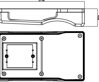
RUBBER - RIGHT
