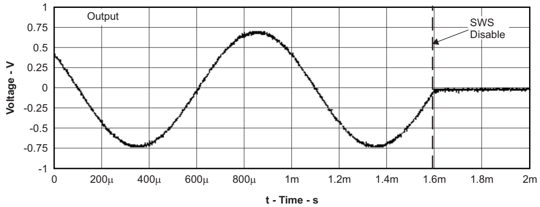
Figure 29. Shutdown Time
