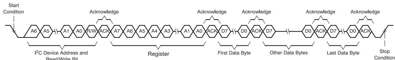
Figure 44. Multiple-Byte Write Transfer
