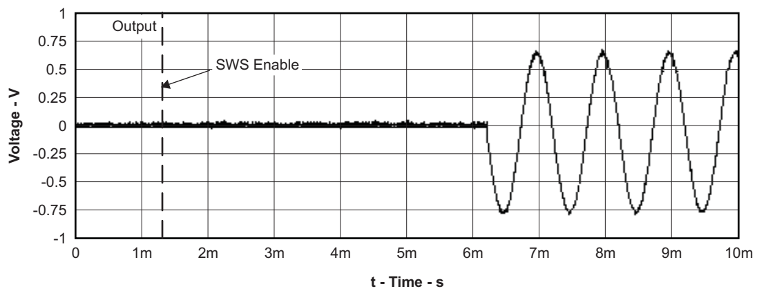
Figure 30. Startup Time
