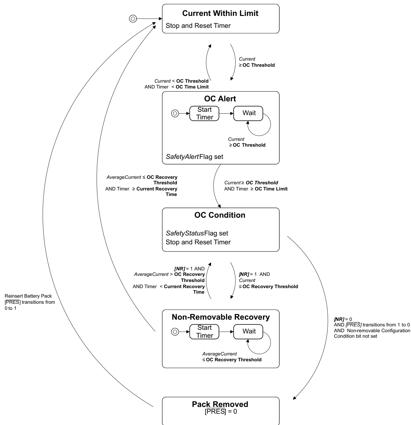
Figure 2-2. OC Protection
