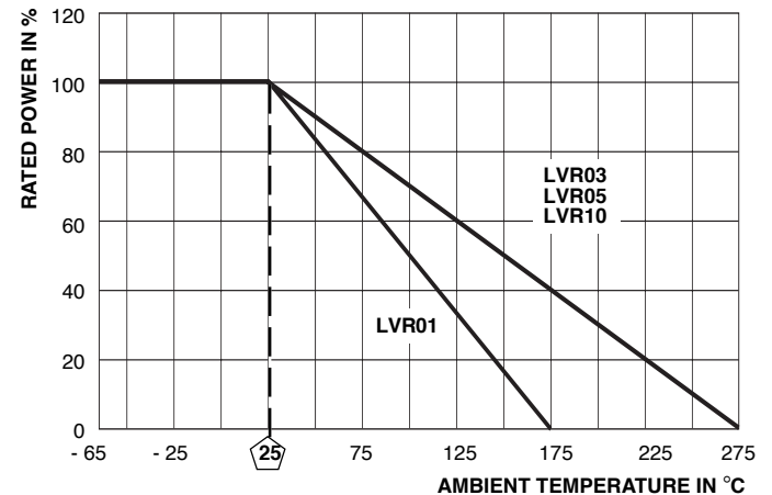
Derating
