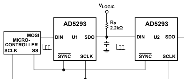
Figure 45. Daisy-Chain Configuration Using SDO
