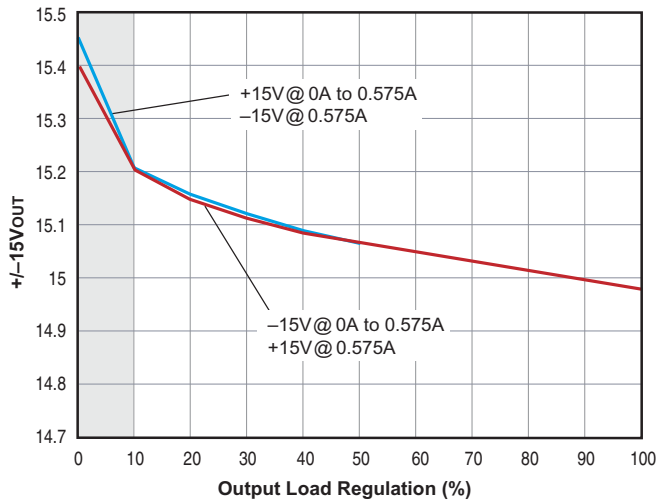
Figure 4. Output Voltage Accuracy vs. Imbalanced Loading
