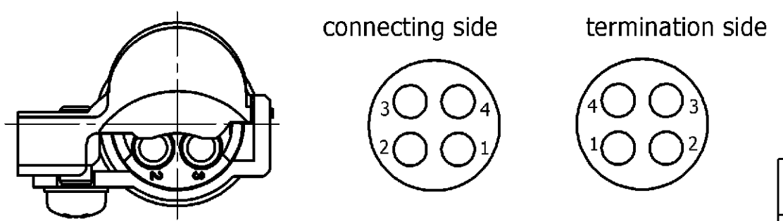
Contact arrangement
