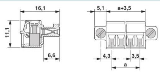
Dimensioned drawing
