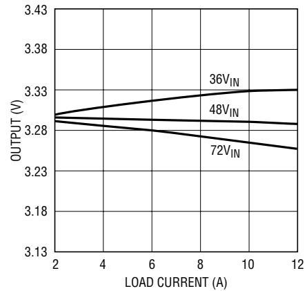
Regulation vs Load Current
