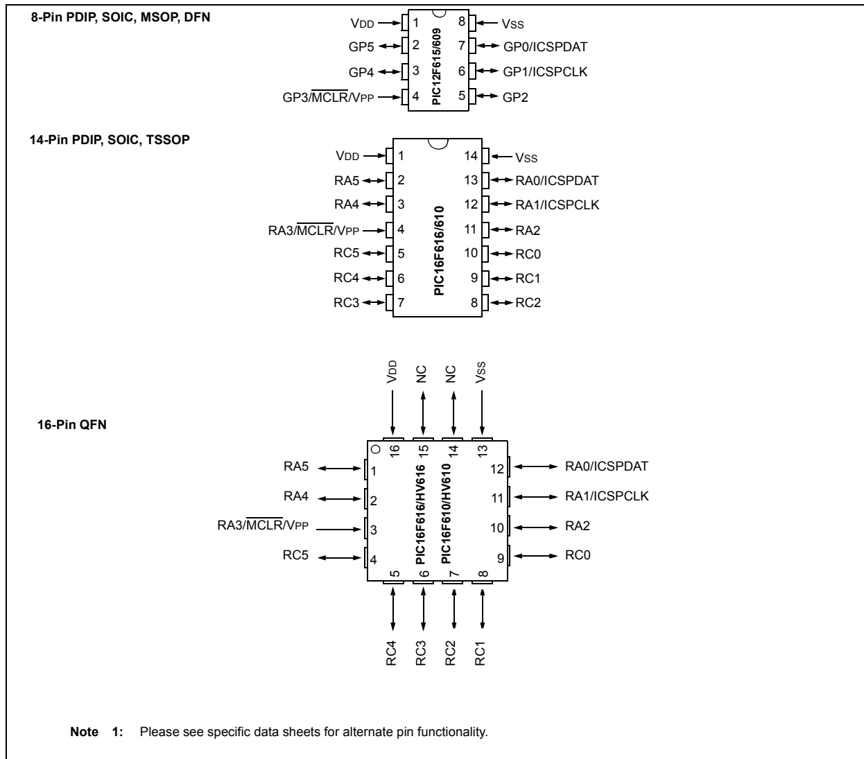
FIGURE 2-1: 8-PIN, 14-PIN, AND 16-PIN PROGRAMMING PINS DIAGRAM FOR PIC12F609/12F615/16F610/16F616 (1)
