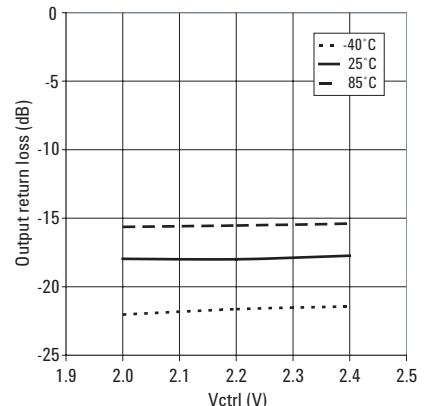
Figure 23. S22 vs Vctrl and temperature
