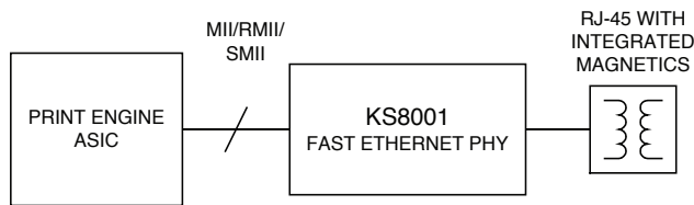
Block Diagram: Network Printer Application
