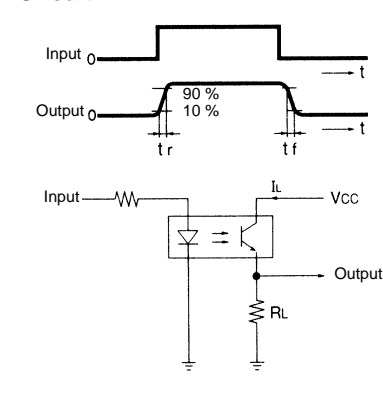
Response Time Measurement Circuit
