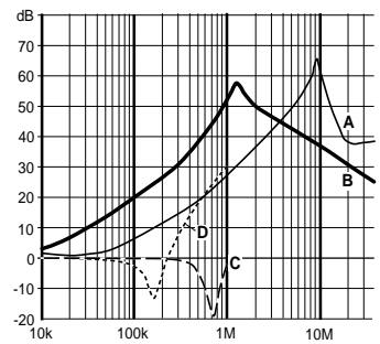
FN 422 1 amp types
