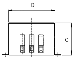
Housing B13 (Connection /33)
