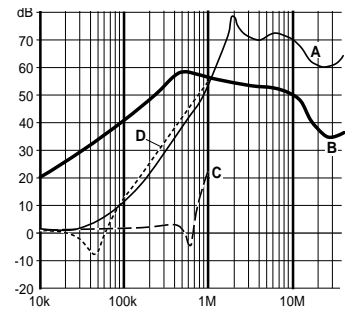
FN 420 6.5 amp types
