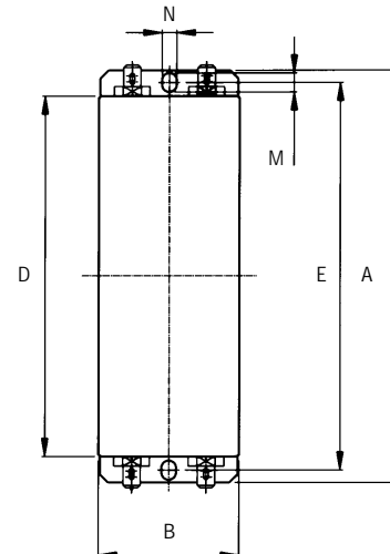
Housing B22
