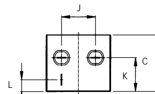
Housing B22
