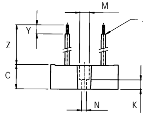
Housing KB1
