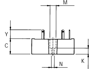
Housing KB2
