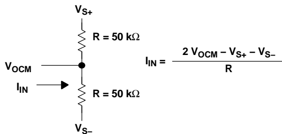
Equivalent Input Circuit for V_{OCM} Figure 101
