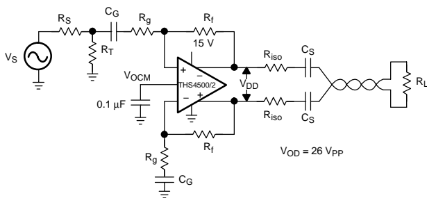
Fully Differential Line Driver With High Output Swing Figure 99
