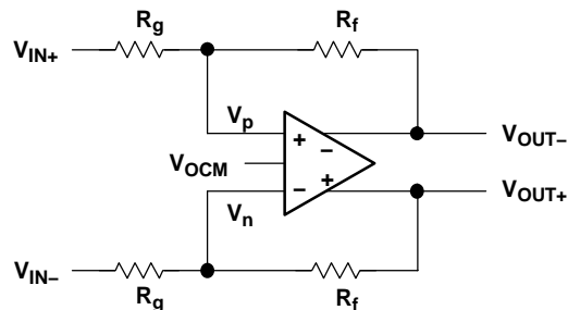
Diagram For Input Common-Mode Range Equations Figure 95
