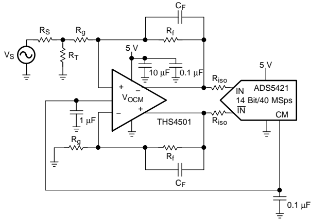
Using the THS4501 With the ADS5421 Figure 98
