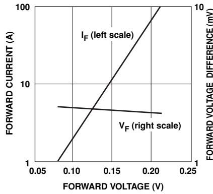
Figure 2. Forward Voltage Match.
