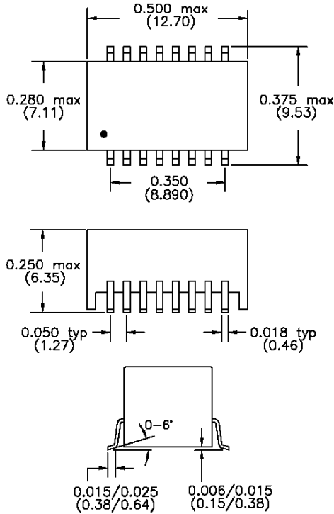
N5 Package
