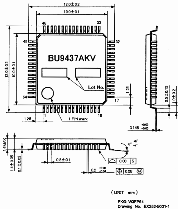
Figure 1. External dimension
