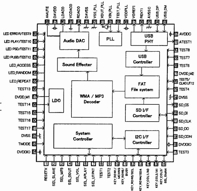
Figure 2. Block diagram
