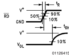
FIGURE 9. TRI-STATE Test Circuits and Waveforms
