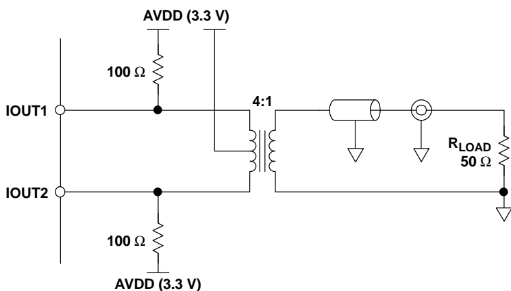
Figure 52. Driving a Doubly Terminated 50- \Omega Cable Using a 4:1 Impedance-Ratio Transformer
