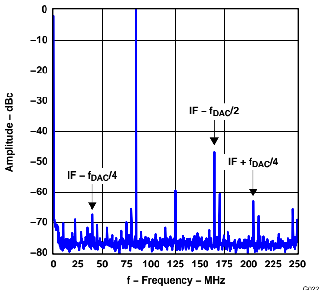
Figure 30. DAC5686 Output Spectrum With f_{\text{DAC}} = 500 \text{ MSPS} , 4\times Interpolation, \text{IF} = 85 \text{ MHz} , and External-Clock Mode
