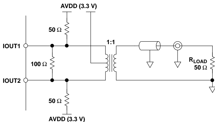
Figure 51. Driving a Doubly Terminated 50- \Omega Cable Using a 1:1 Impedance-Ratio Transformer
