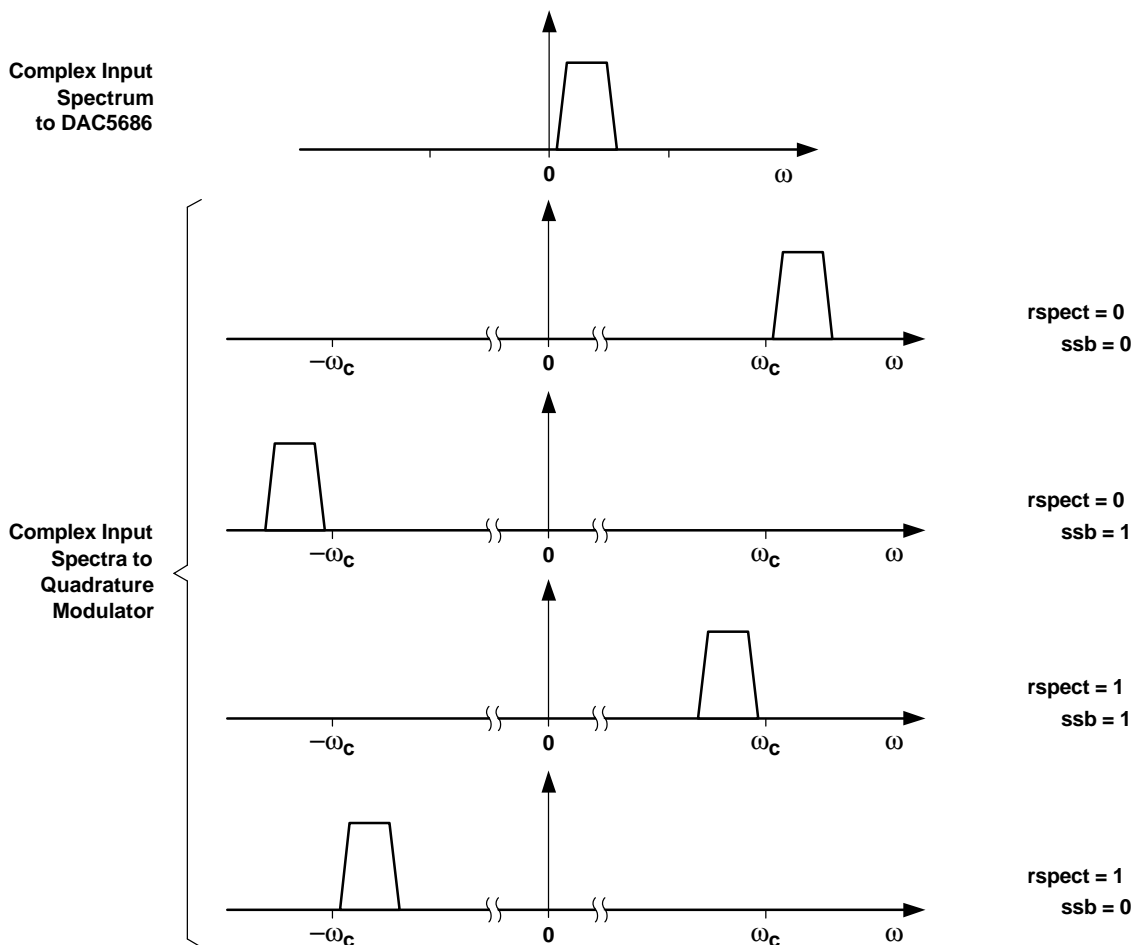
Figure 22. Complex Input Spectrum and DAC Output Spectra
