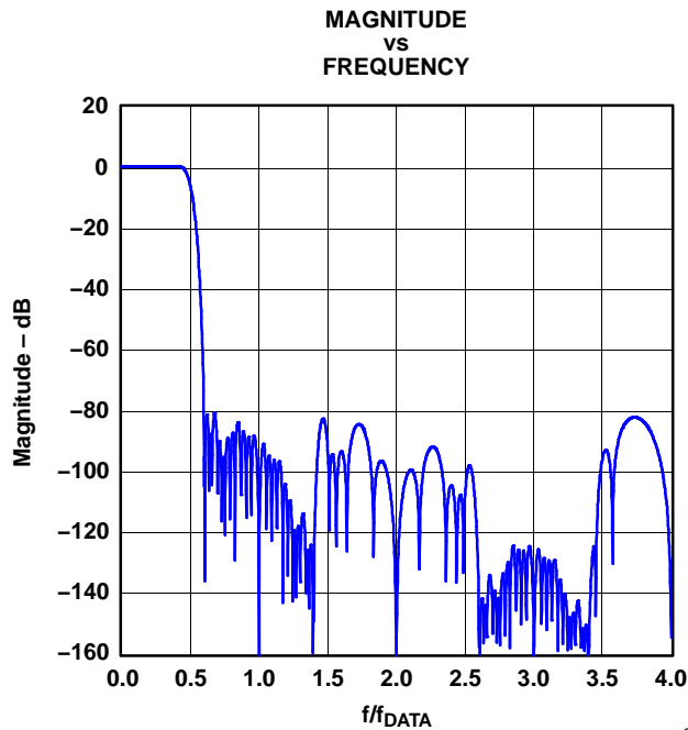
Figure 41. Magnitude Spectrum for 8× Interpolation (dB)
