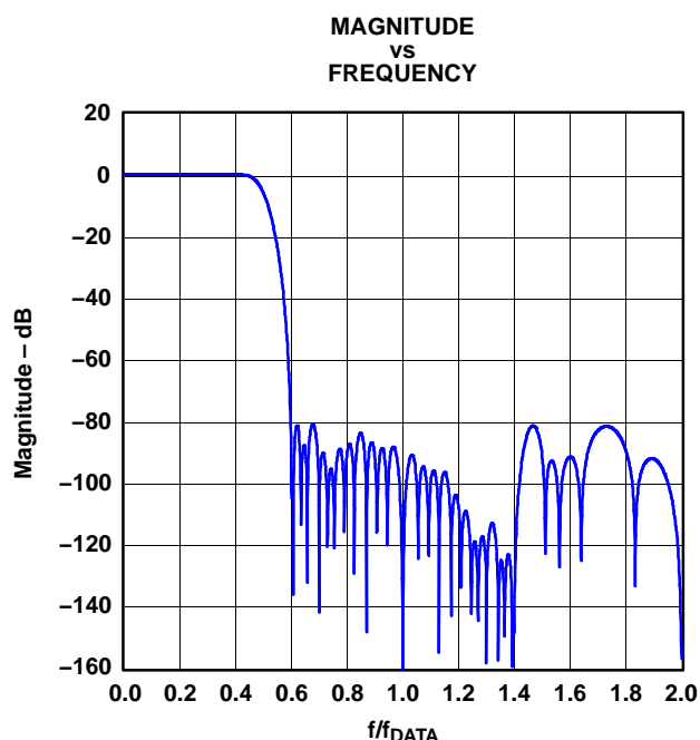
Figure 40. Magnitude Spectrum for 4× Interpolation (dB)
