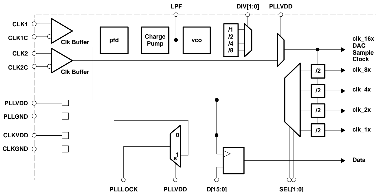
Figure 27. Clock-Generation Architecture
