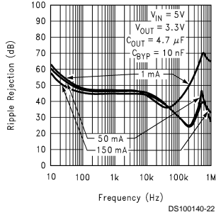
Ripple Rejection
