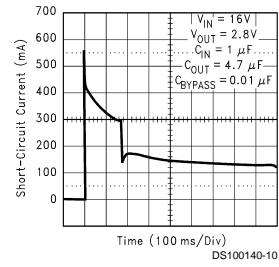
Short-Circuit Current
