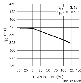
Instantaneous Short Circuit Current
