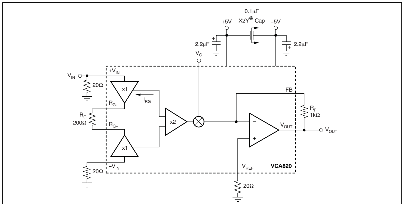
Figure 76. DC-Coupled, A_{\text{VMAX}} = 20\text{dB} , Bipolar Supply Specification and Test Circuit
