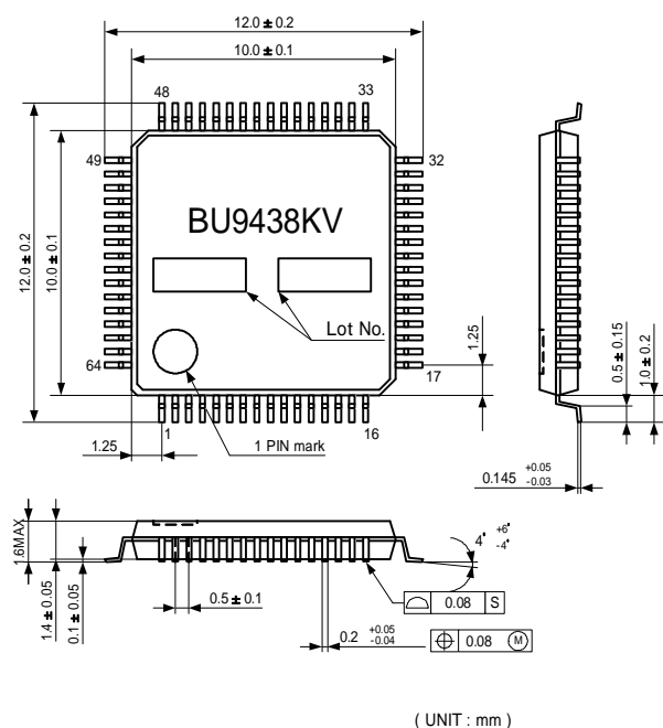
External dimensions · Block diagram
