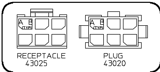
Fig. 1 CONNECTOR PATTERN
