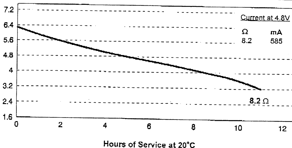
Typical Discharge Characteristics
