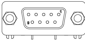
FEMALE, 9 CONTACT D-SUB CONNECTOR
