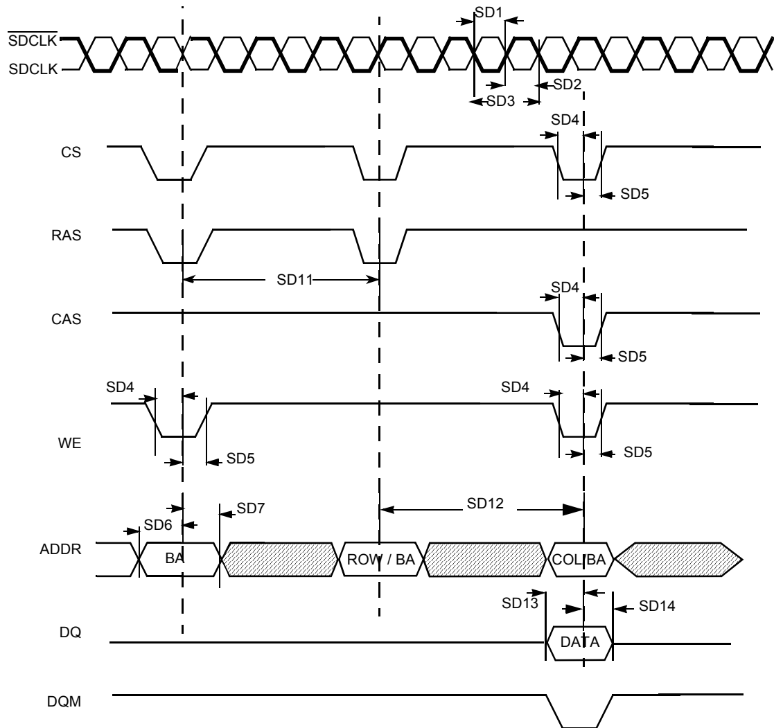
Figure 35. SDR SDRAM Write Cycle Timing Diagram
