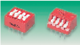
Rocker: H = 7.5, W = 9.5 Pins = 3.96 0.51 0.31 Lever Key: H = 7.14, W = 9.5 Pins = 3.96 0.51 0.31
