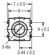
Terminal Arrangement (Top view)
