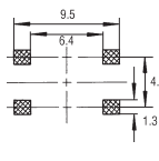
PCB footprint
