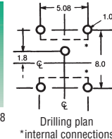
Drilling plan *internal connections
