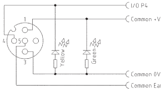
8 Way Top Mount M12 Splitter Box Integral Cable Single I/O
