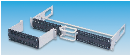
Wall Mounting H = 58, W = 225, D = 125 Fixing Centres = 210
